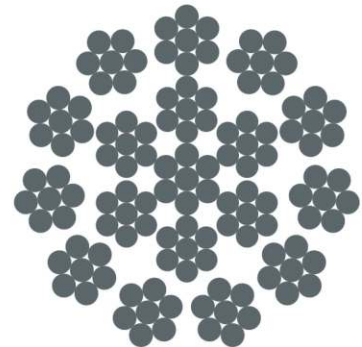
17×7-WSC
