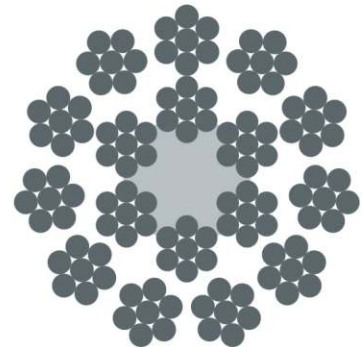
17×7-FC
