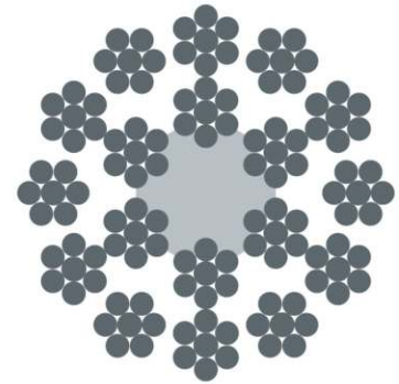
18×7-FC
