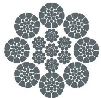
8×K26WS-IWRC(7x19S)
