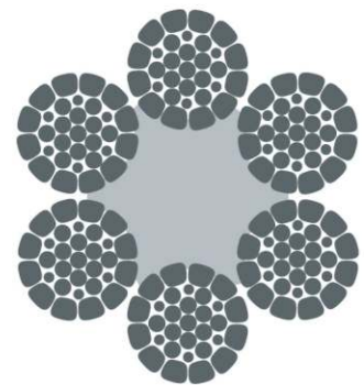
6×K31WS-FC
